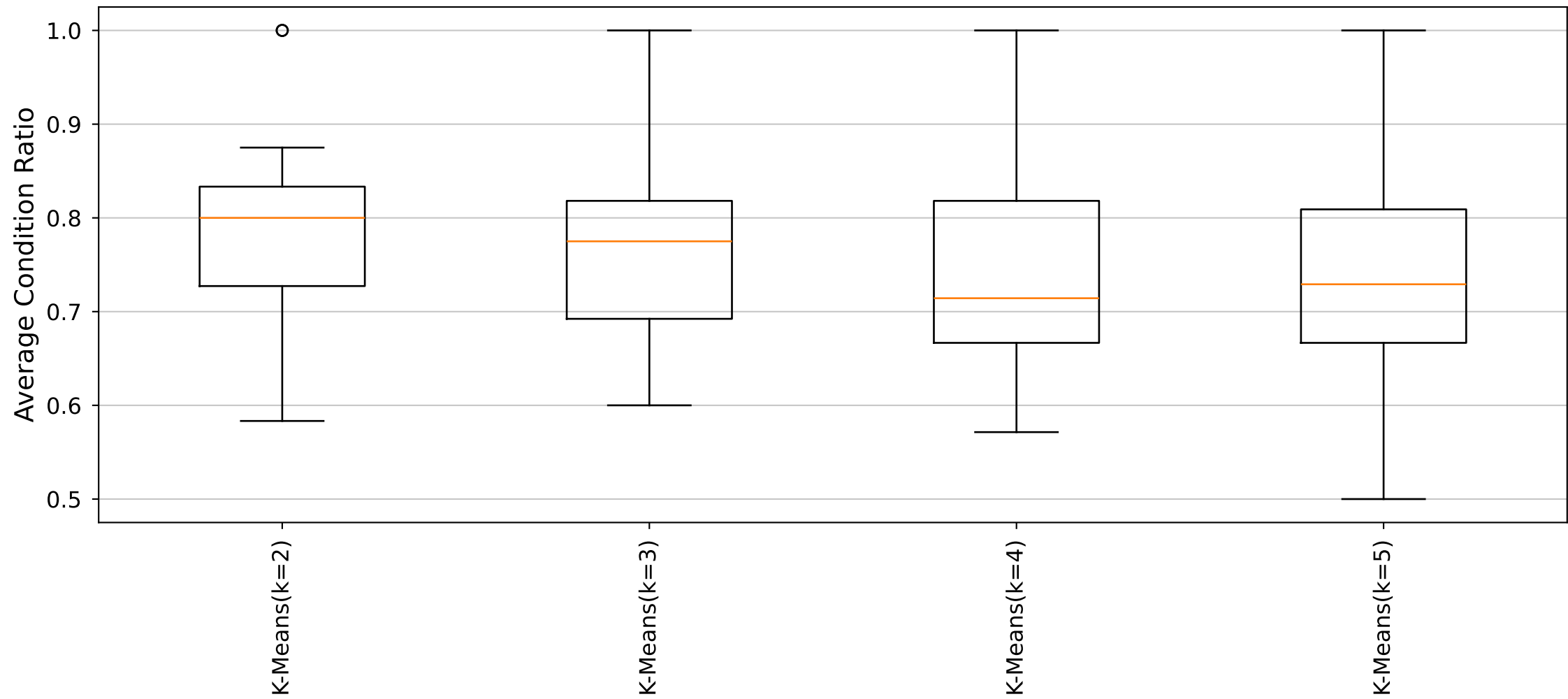
YARA Rules Average Condition Ratio Distribution (Cluster42_Size5 dataset)
